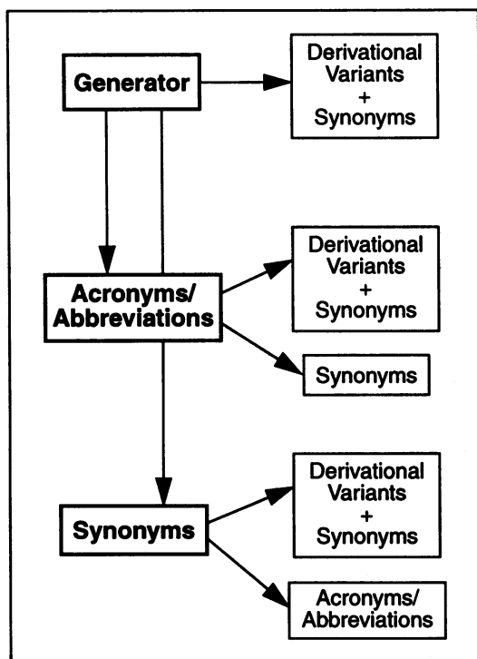
Figure 2. Variant generation
