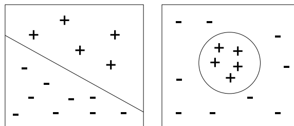
Figure 1: Instance sets
