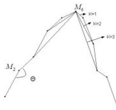
Fig. 1. Multiple Open Triangles and the angles
