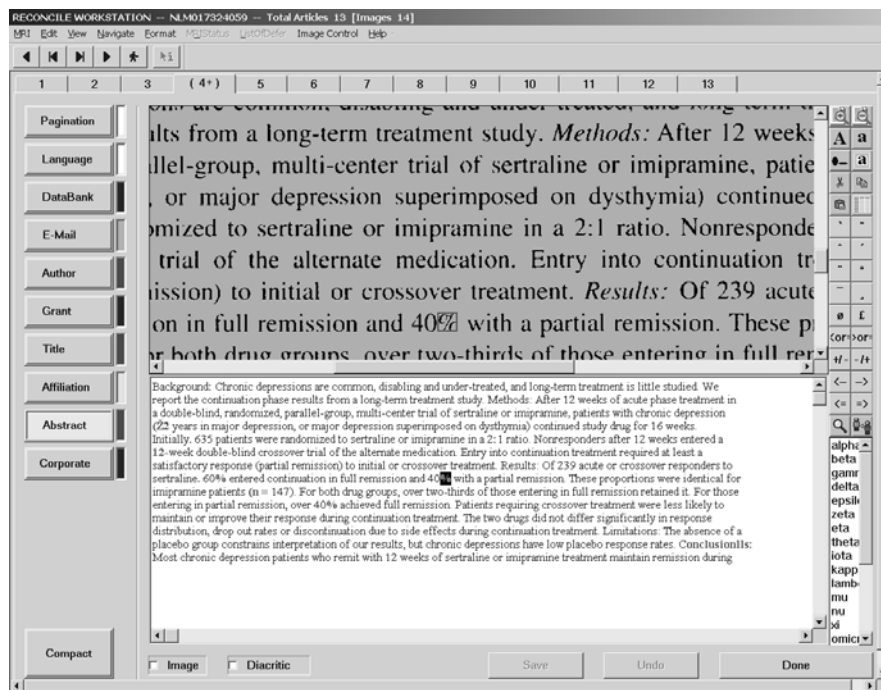
Figure 3 Split view shows both the bitmapped image and corresponding text. Low confidence characters are highlighted in the text window.
