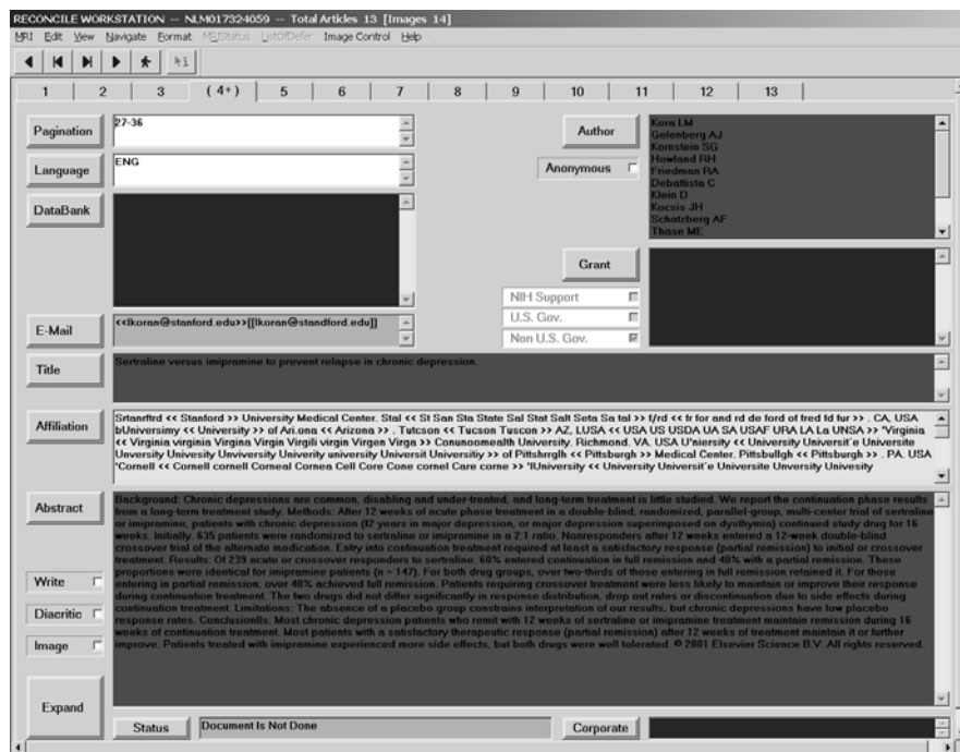
Figure 2 General view for all bibliographic fields in an article.
