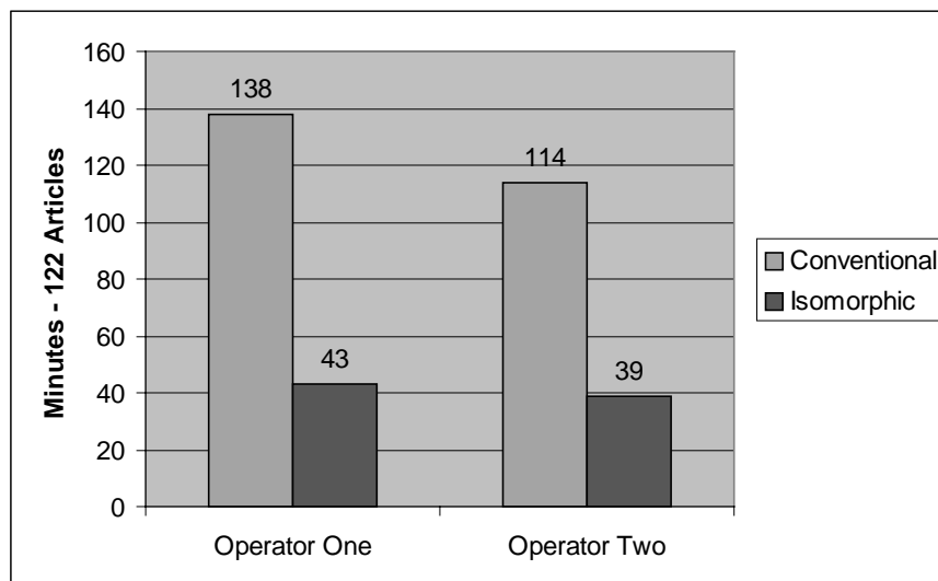
Figure 7 – Time taken to correct OCR errors using conventional and Isomorphic methods.
